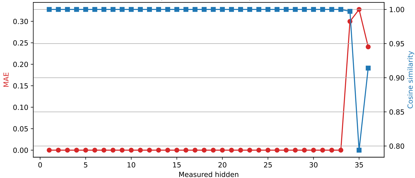
SmolLM3-3B | Quantized layer 33 | float16 → int2
