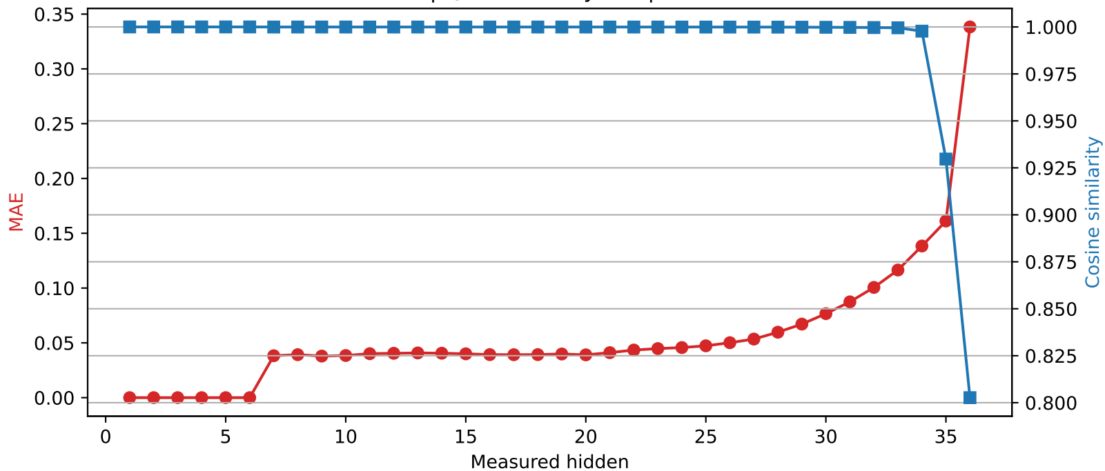
SmolLM3-3B | Quantized layer 6 | float16 → int2
