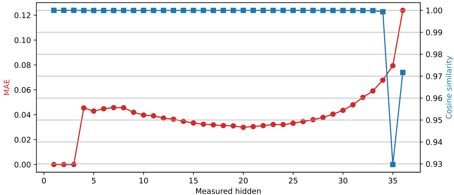
SmolLM3-3B | Quantized layer 3 | float16 → int2
