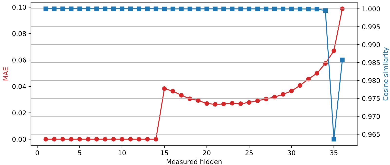
SmolLM3-3B | Quantized layer 14 | float16 \rightarrow int2
