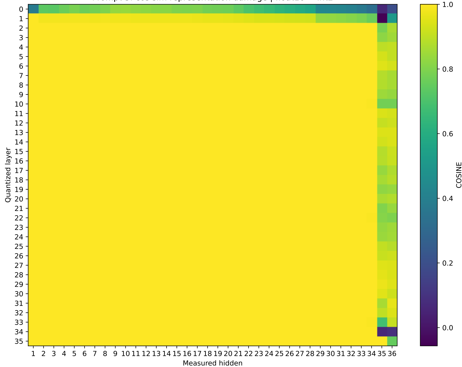
SmolLM3-3B Prompt 3: cos sim representation damage | float16 → int2
