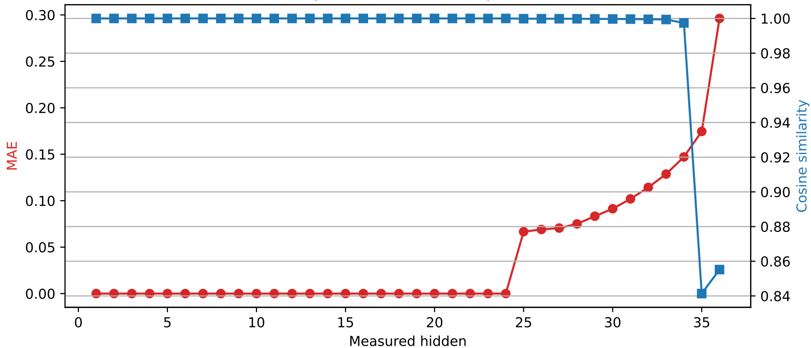
SmolLM3-3B | Quantized layer 24 | float16 → int2
