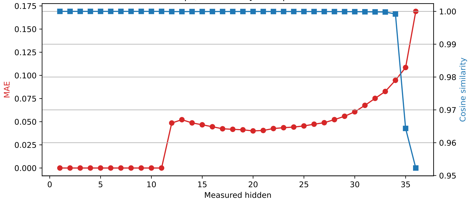
SmolLM3-3B | Quantized layer 11 | float16 \rightarrow int2
