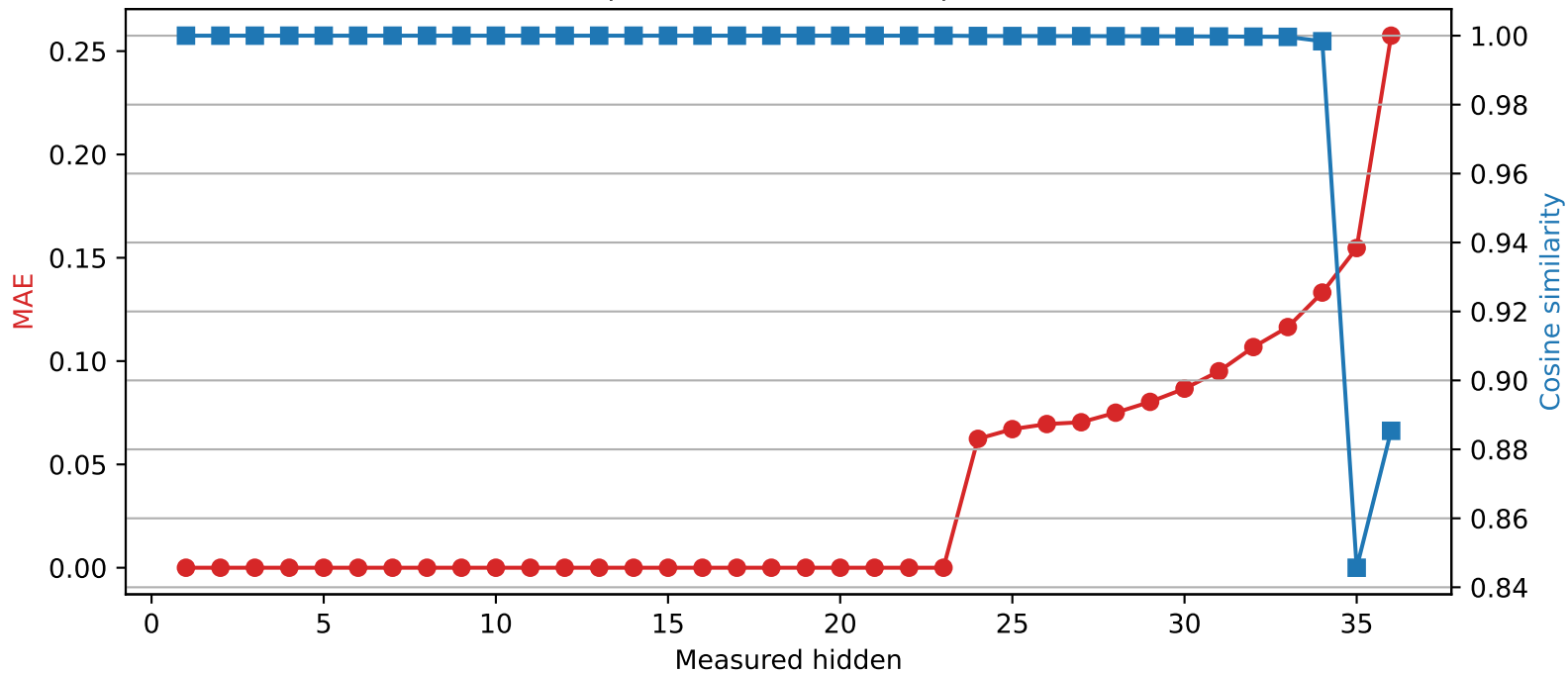
SmolLM3-3B | Quantized layer 23 | float16 → int2
