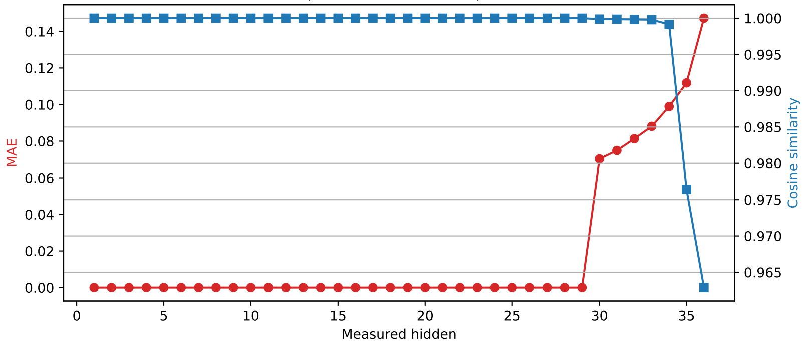
SmolLM3-3B | Quantized layer 29 | float16 → int2
