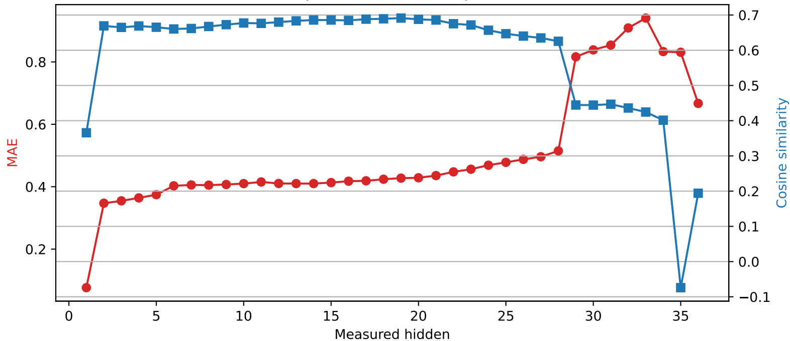
SmolLM3-3B | Quantized layer 0 | float32 → int2
