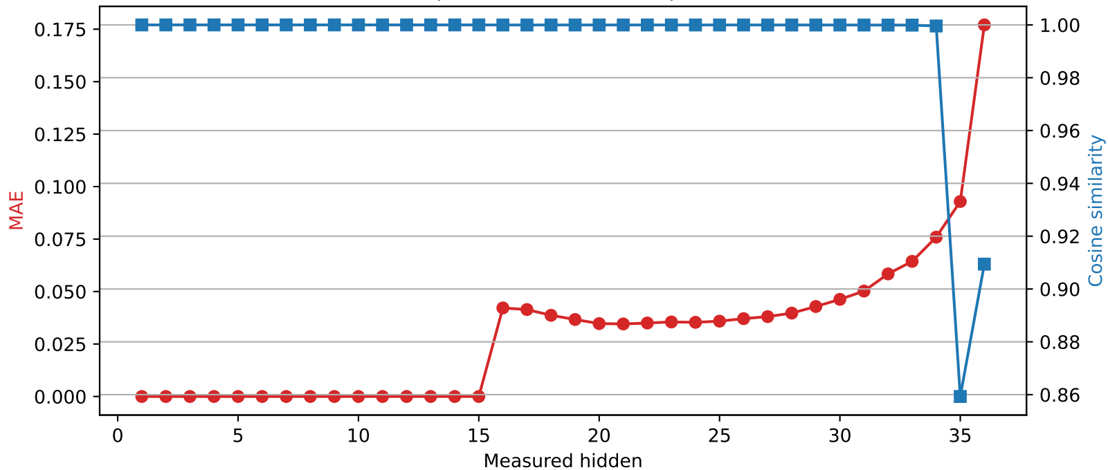
SmolLM3-3B | Quantized layer 15 | float32 → int2
