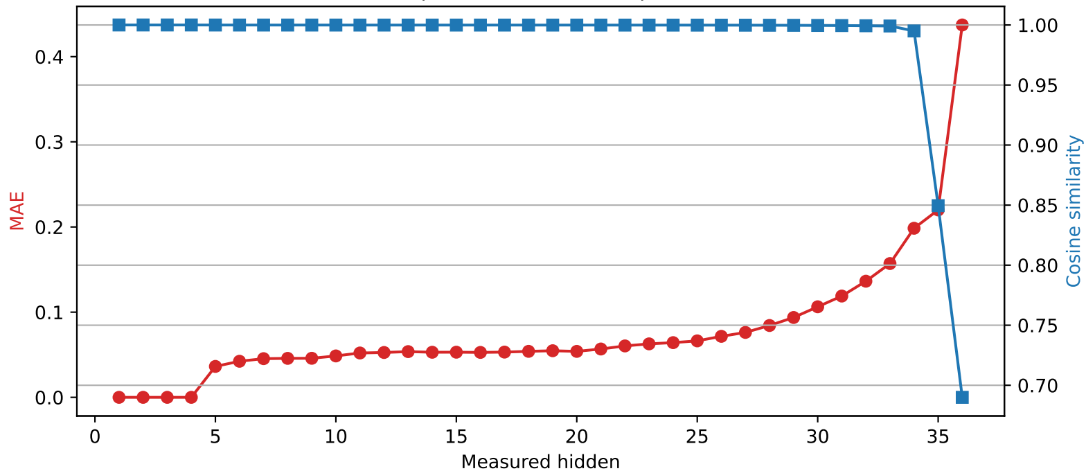
SmolLM3-3B | Quantized layer 4 | float32 → int2
