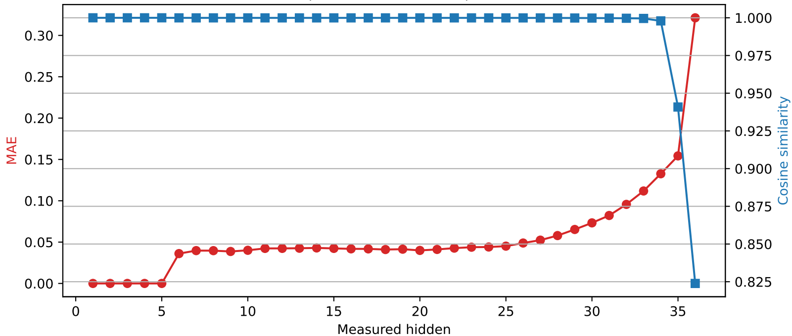
SmolLM3-3B | Quantized layer 5 | float32 → int2
