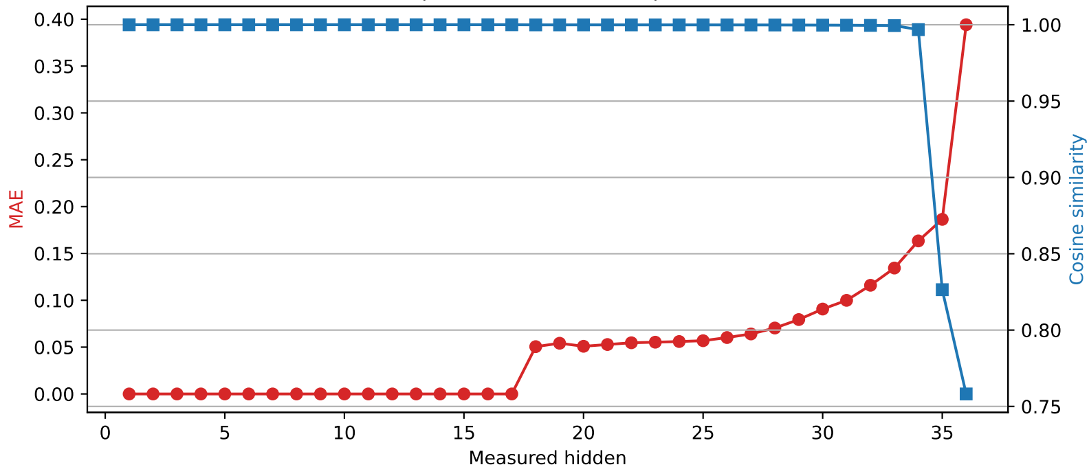
SmolLM3-3B | Quantized layer 17 | float32 \rightarrow int2
