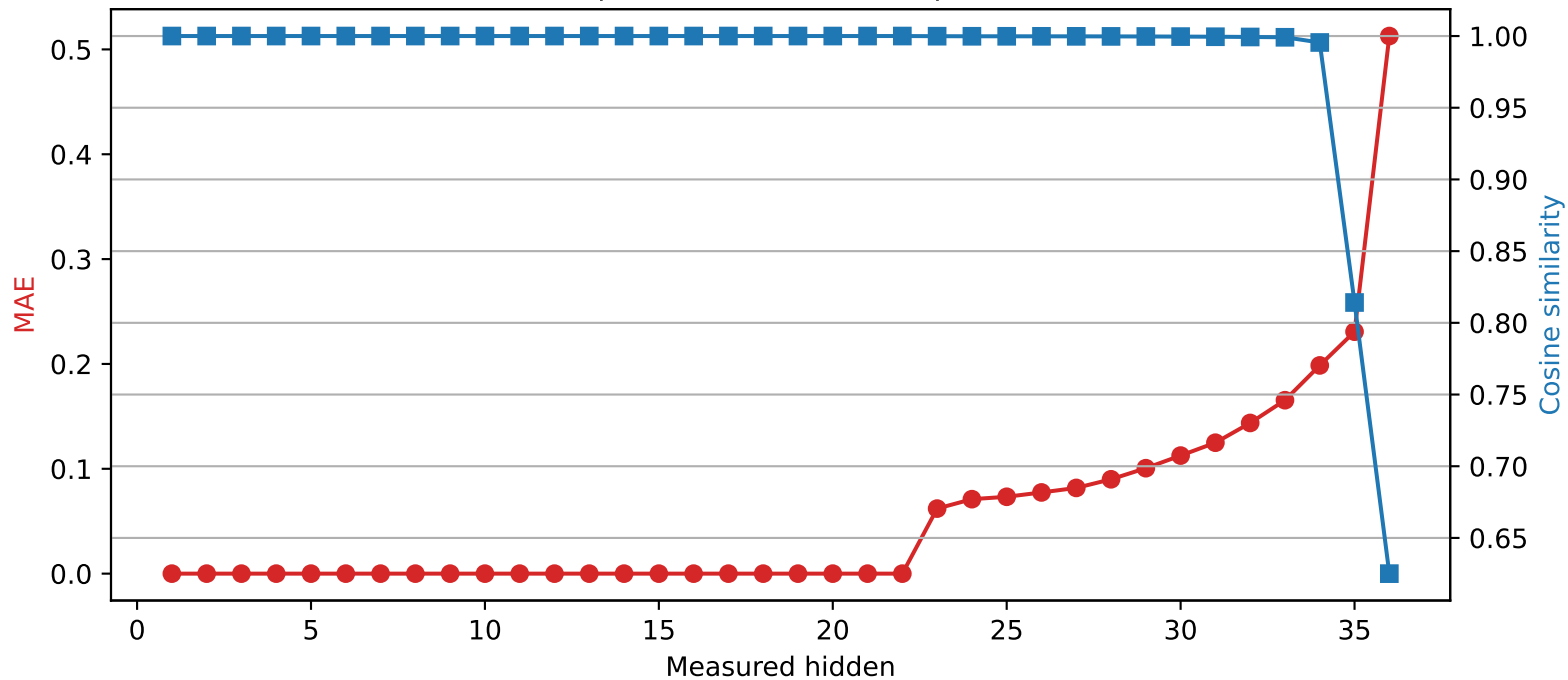
SmolLM3-3B | Quantized layer 22 | float32 → int2
