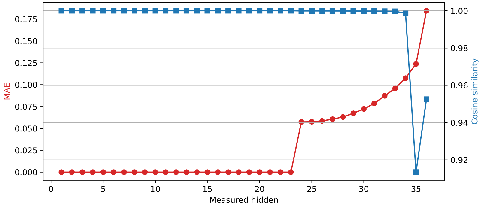
SmolLM3-3B | Quantized layer 23 | float32 → int2
