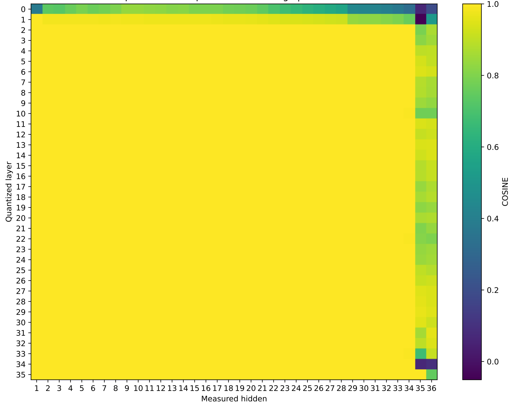
SmolLM3-3B Prompt 3: cos sim representation damage | float32 → int2
