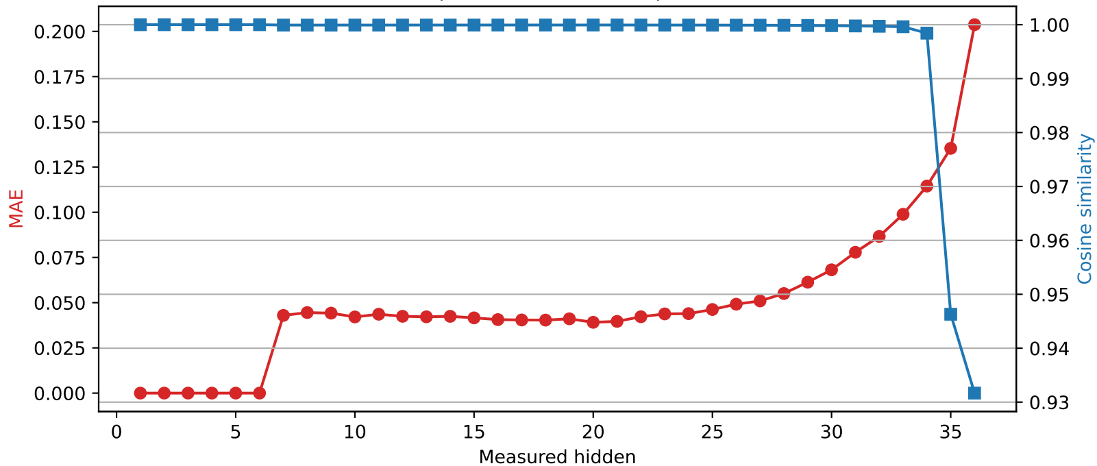
SmolLM3-3B | Quantized layer 6 | float32 \rightarrow int2
