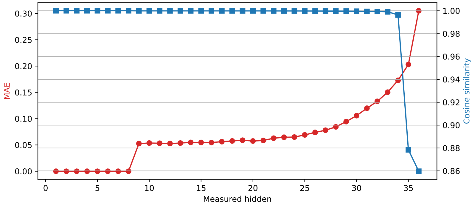
SmolLM3-3B | Quantized layer 8 | float32 → int2
