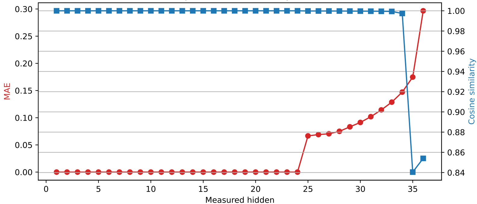
SmolLM3-3B | Quantized layer 24 | float32 → int2
