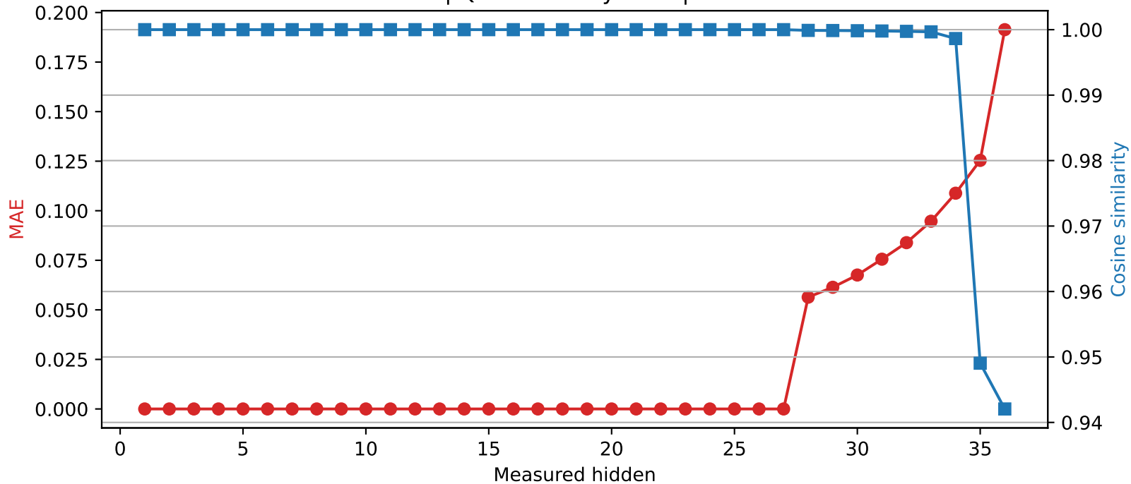
SmolLM3-3B | Quantized layer 27 | float32 → int2
