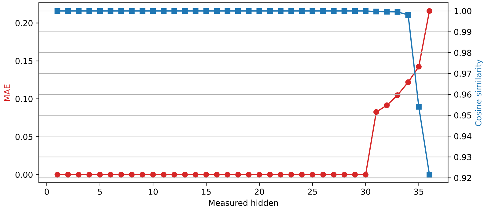
SmolLM3-3B | Quantized layer 30 | float32 \rightarrow int2
