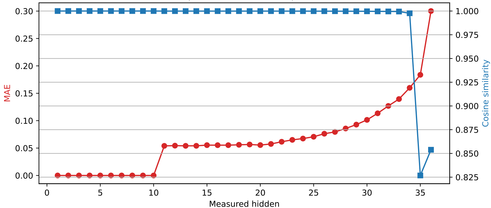
SmolLM3-3B | Quantized layer 10 | float32 → int2
