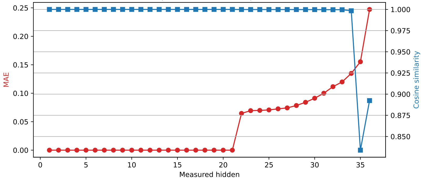
SmolLM3-3B | Quantized layer 21 | float32 \rightarrow int2
