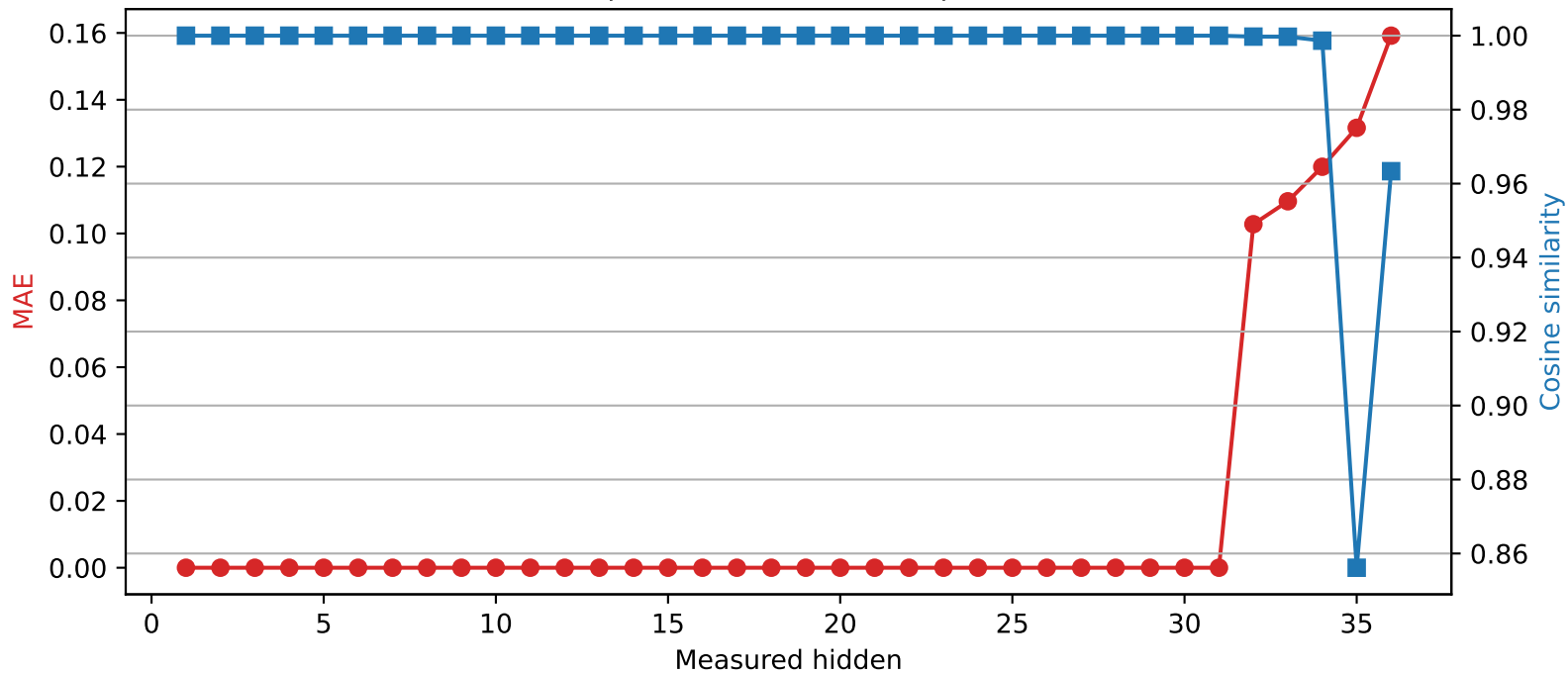
SmolLM3-3B | Quantized layer 31 | float32 → int2
