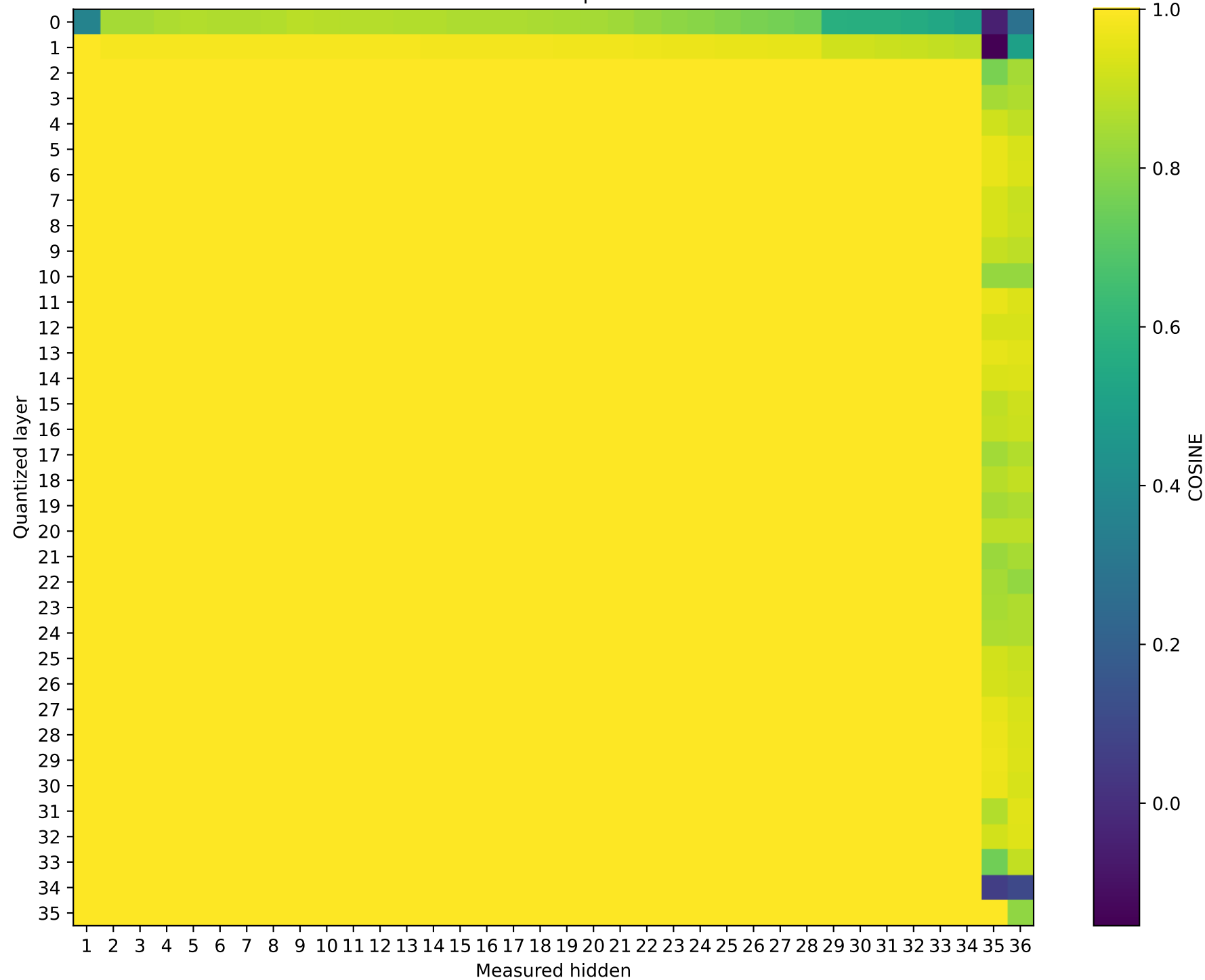
Model: SmolLM3-3B | float64 → int2
