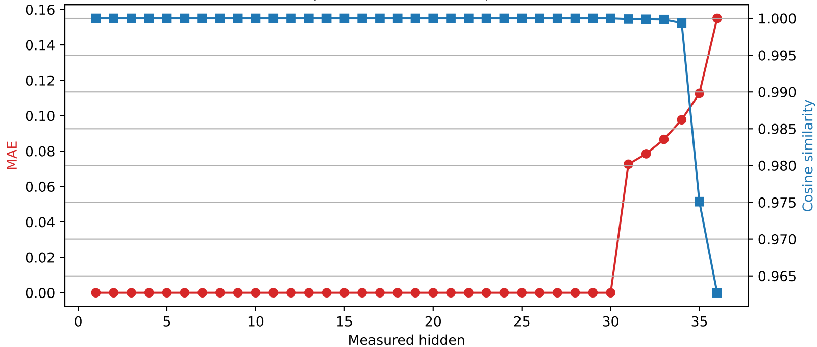
SmolLM3-3B | Quantized layer 30 | float64 → int2
