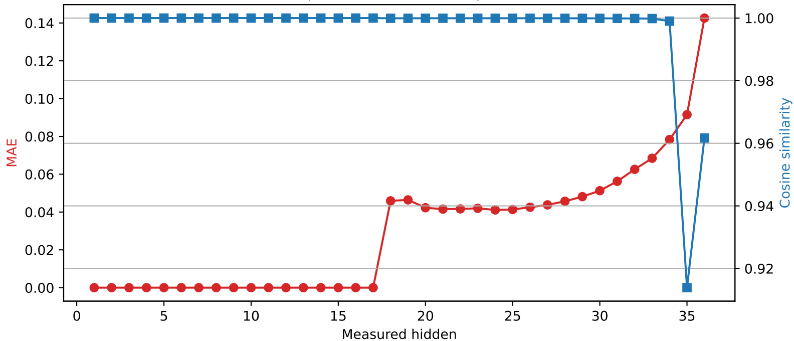
SmolLM3-3B | Quantized layer 17 | float64 → int2
