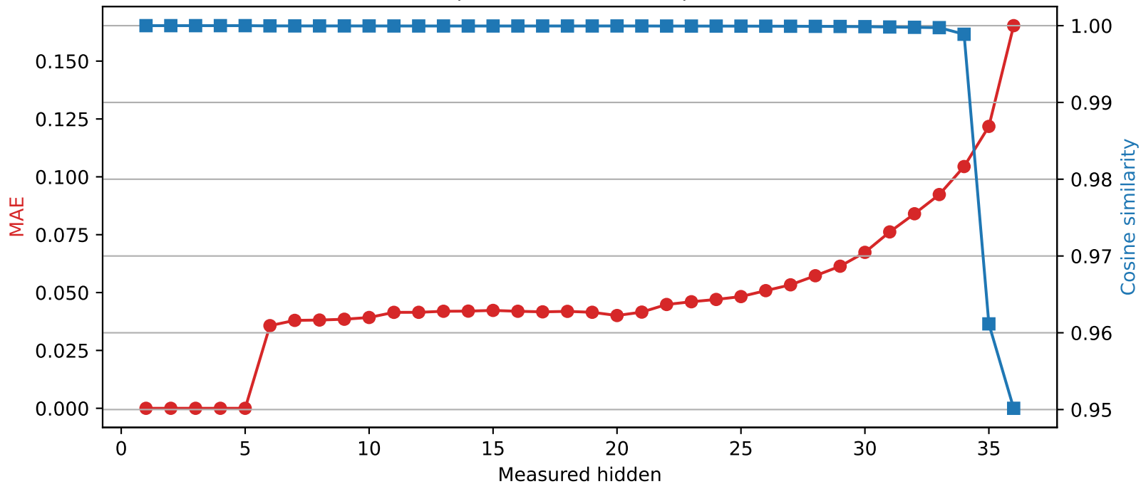
SmolLM3-3B | Quantized layer 5 | float64 → int2
