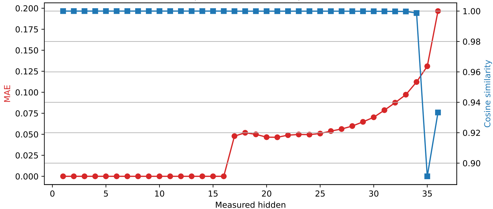
SmolLM3-3B | Quantized layer 16 | float64 → int2
