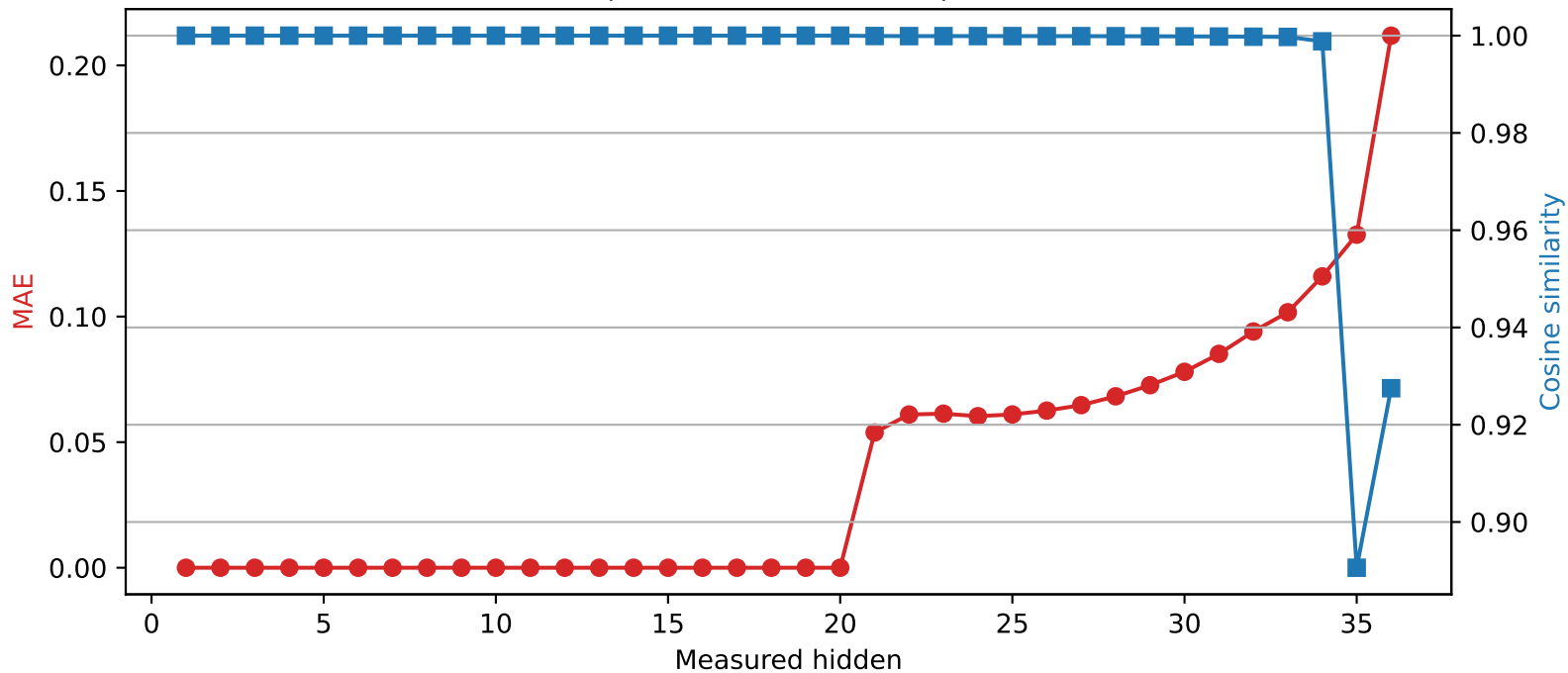
SmolLM3-3B | Quantized layer 20 | float64 → int2
