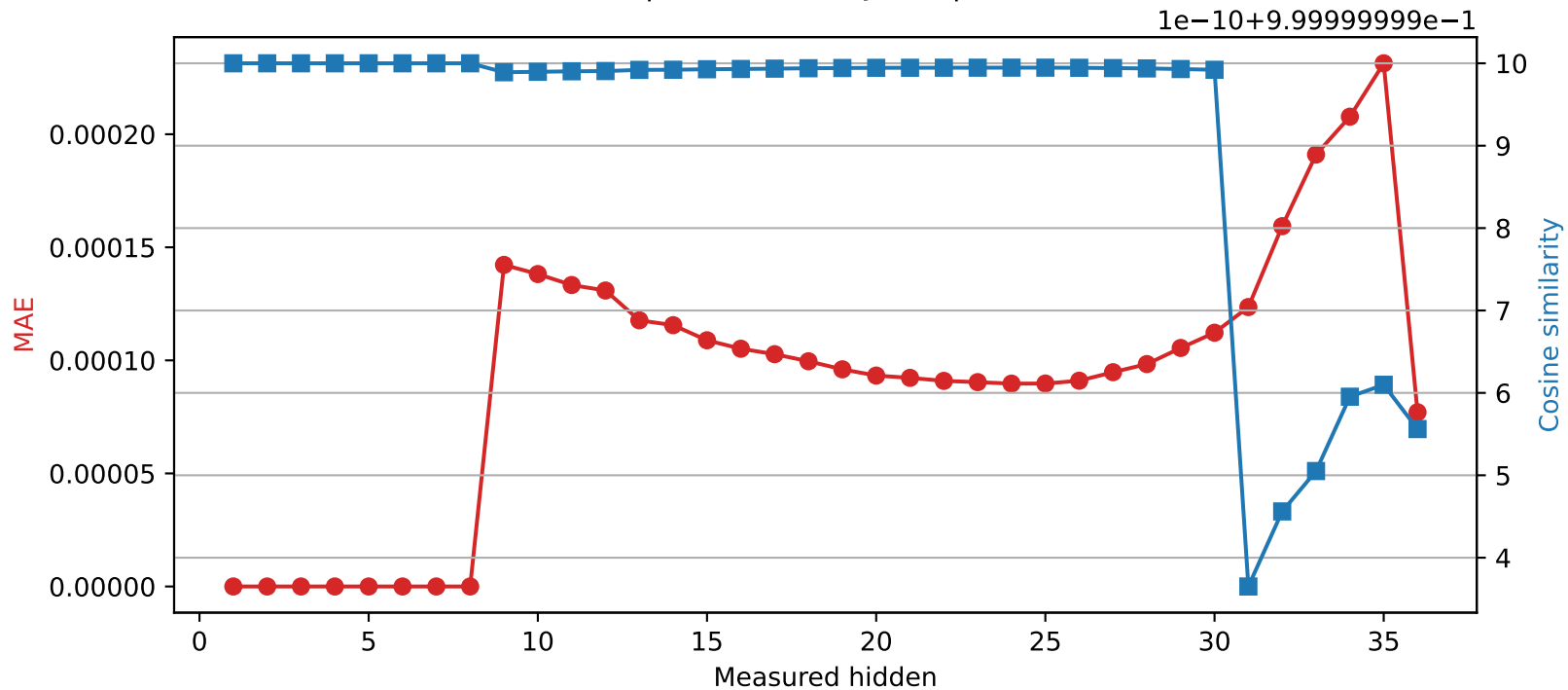
Qwen2.5-3B | Quantized layer 8 | float32 → int16
