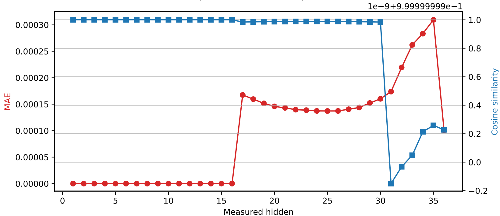
Qwen2.5-3B | Quantized layer 16 | float32 → int16
