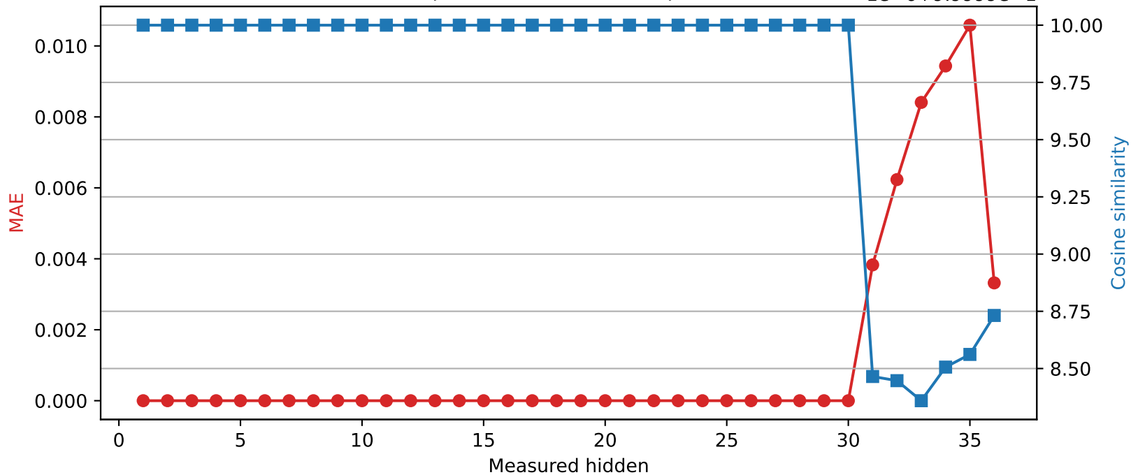
Qwen2.5-3B | Quantized layer 30 | float32 \rightarrow int16 1e-6 + 9.9999e-1
