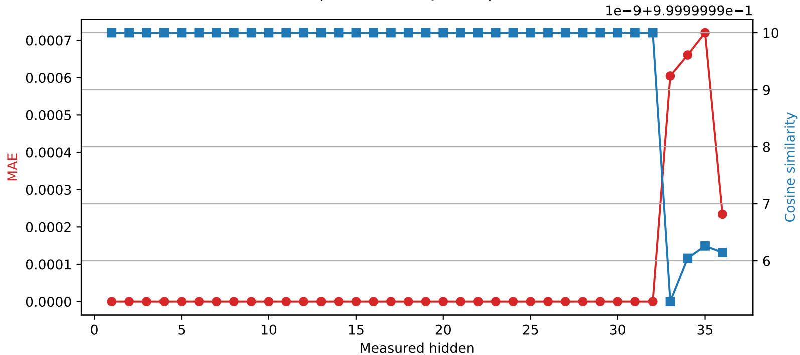
Qwen2.5-3B | Quantized layer 32 | float32 → int16
