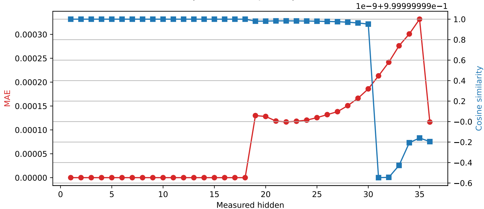
Qwen2.5-3B | Quantized layer 18 | float32 → int16
