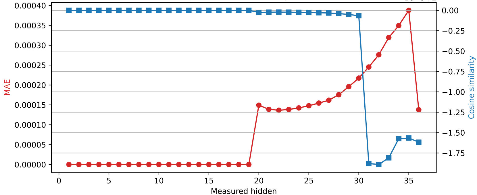
Qwen2.5-3B | Quantized layer 19 | float32 → int16
