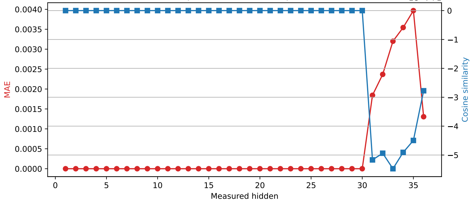
Qwen2.5-3B | Quantized layer 30 | float32 → int16
