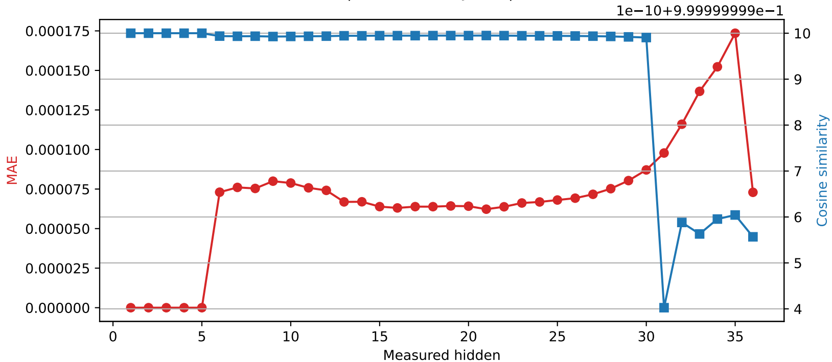
Qwen2.5-3B | Quantized layer 5 | float32 → int16
