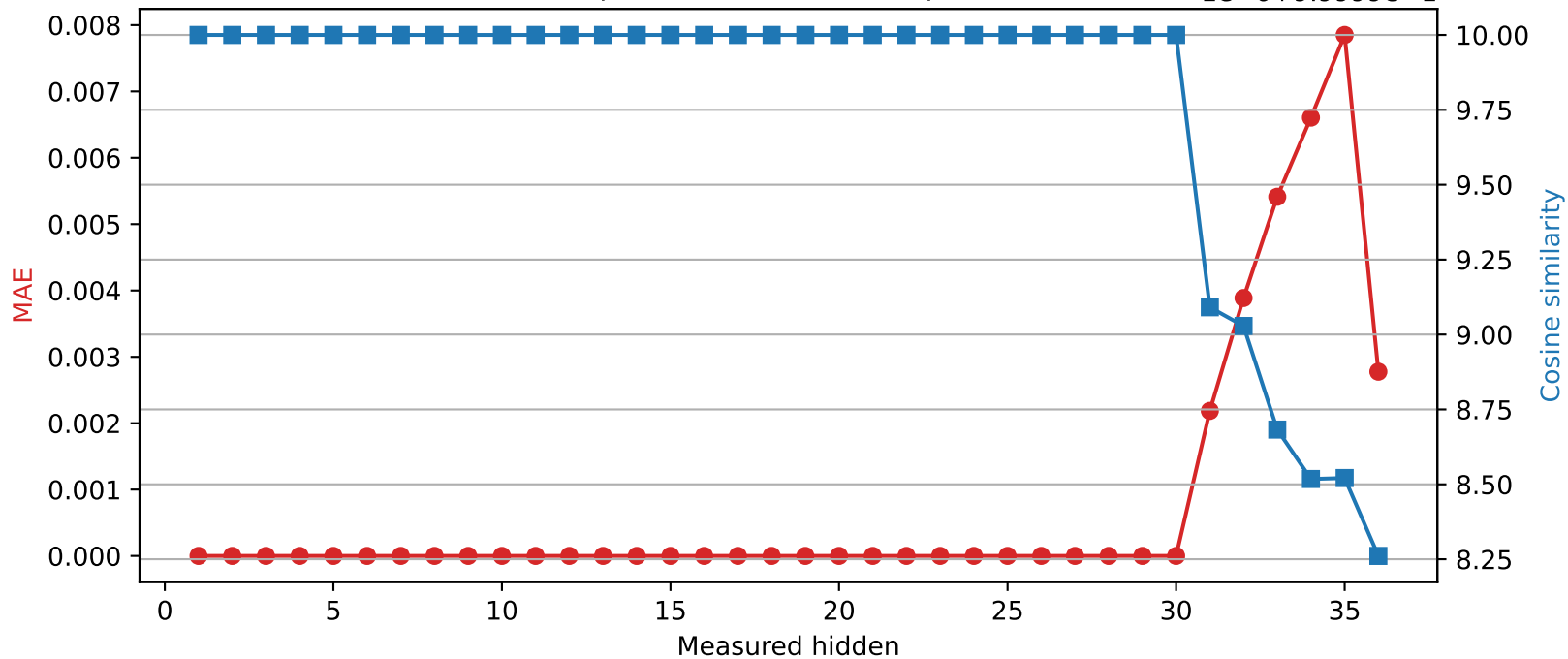
Qwen2.5-3B | Quantized layer 30 | float32 \rightarrow int16 1e-6+9.9999e-1
