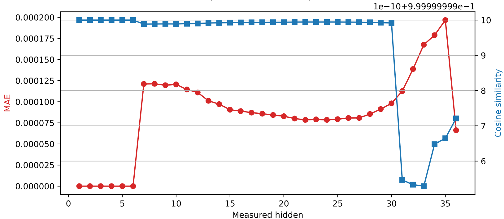
Qwen2.5-3B | Quantized layer 6 | float32 → int16
