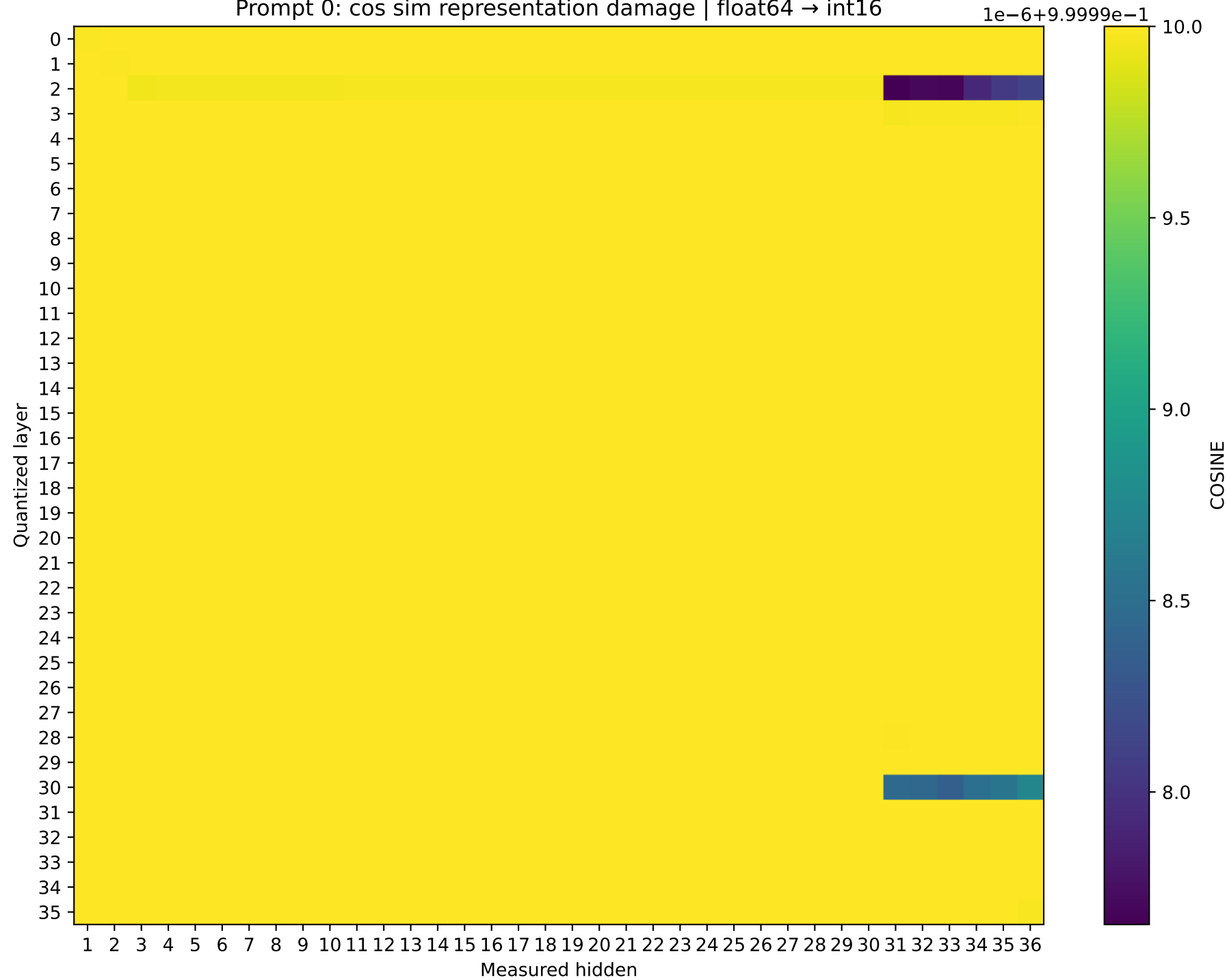
Qwen2.5-3B Prompt 0: cos sim representation damage | float64 → int16
