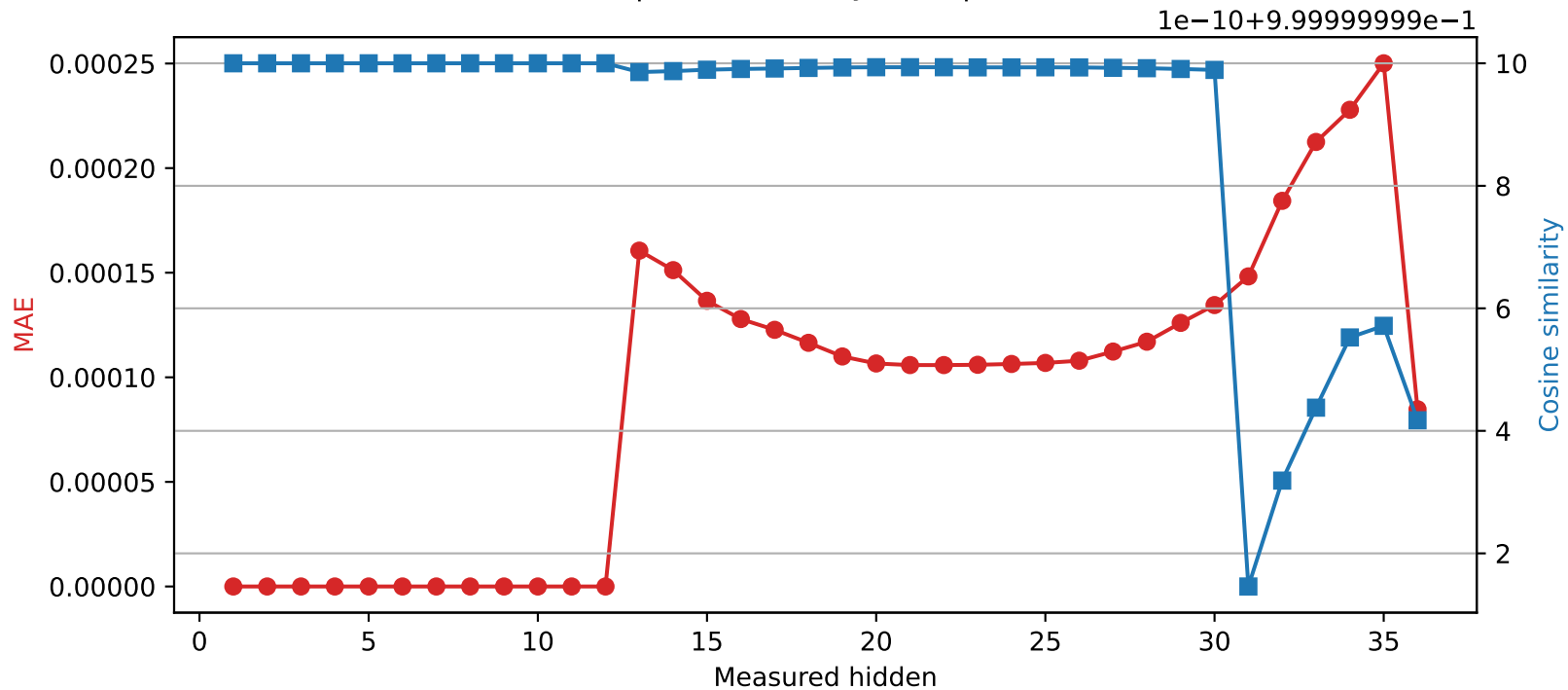
Qwen2.5-3B | Quantized layer 12 | float64 → int16
