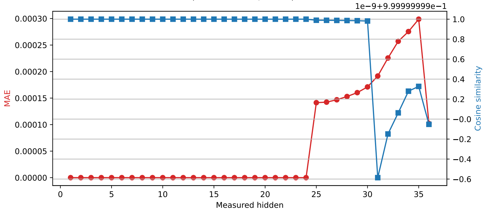
Qwen2.5-3B | Quantized layer 24 | float64 → int16
