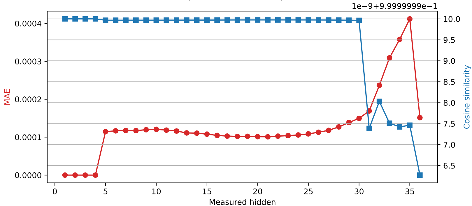
Qwen2.5-3B | Quantized layer 4 | float64 → int16
