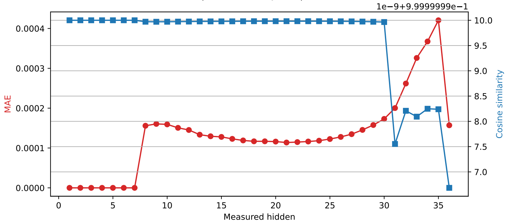
Qwen2.5-3B | Quantized layer 7 | float64 → int16
