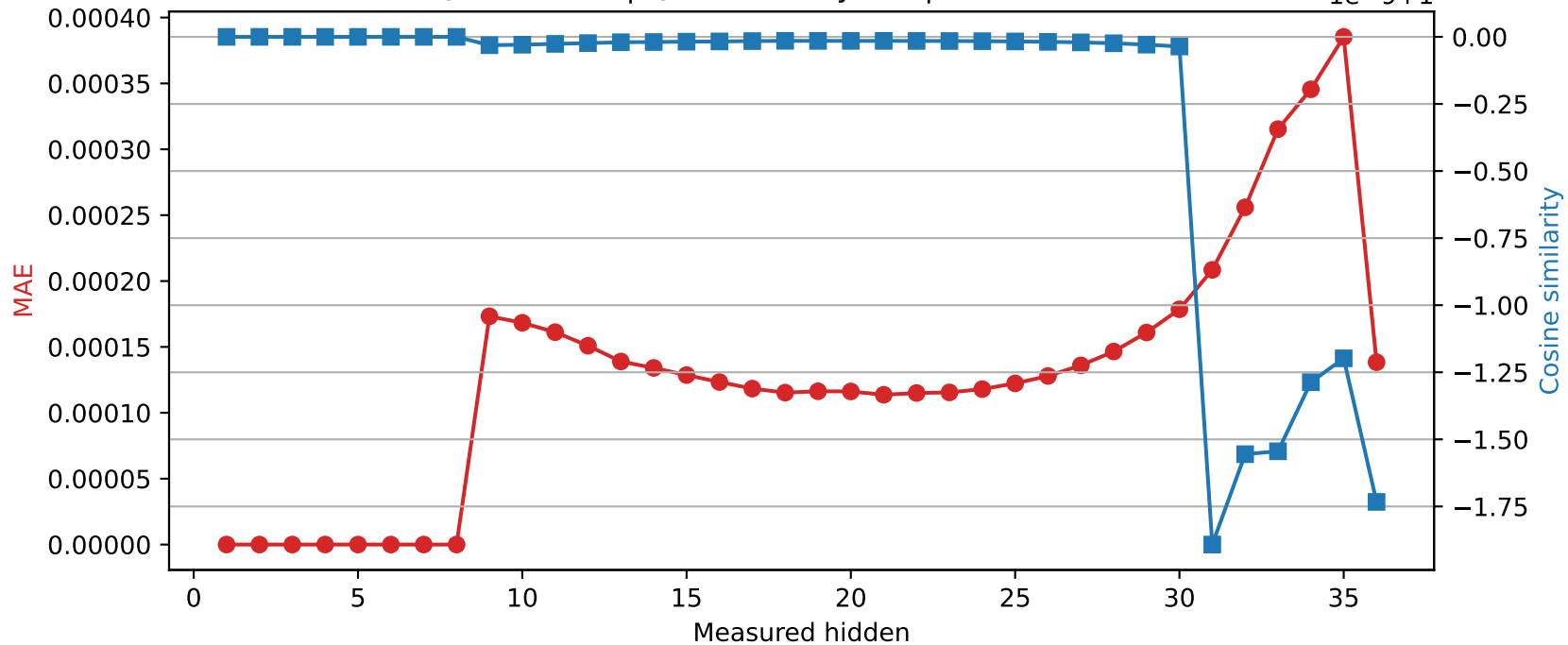
Qwen2.5-3B | Quantized layer 8 | float64 → int16
