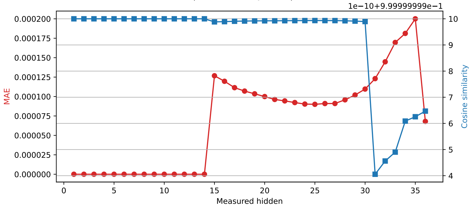
Qwen2.5-3B | Quantized layer 14 | float64 → int16
