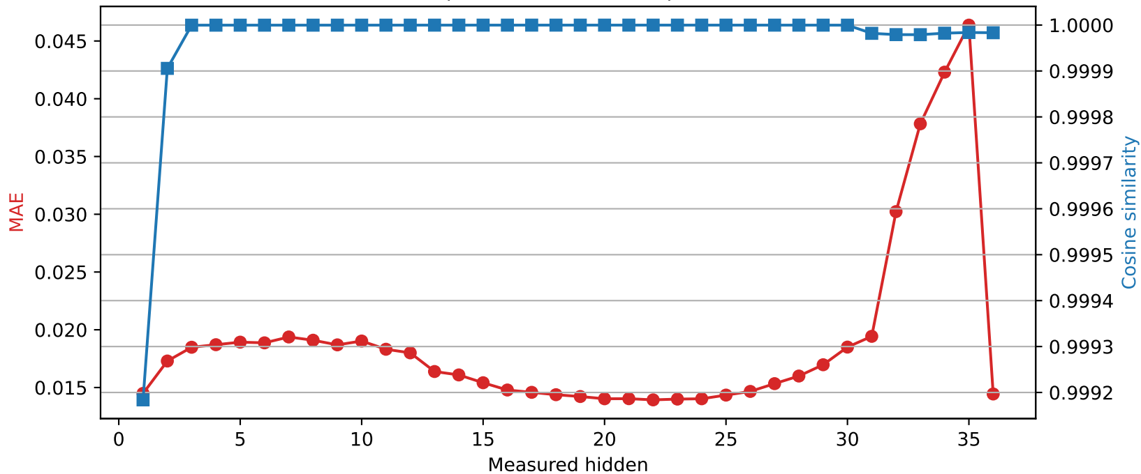
Qwen2.5-3B | Quantized layer 0 | float16 → int8
