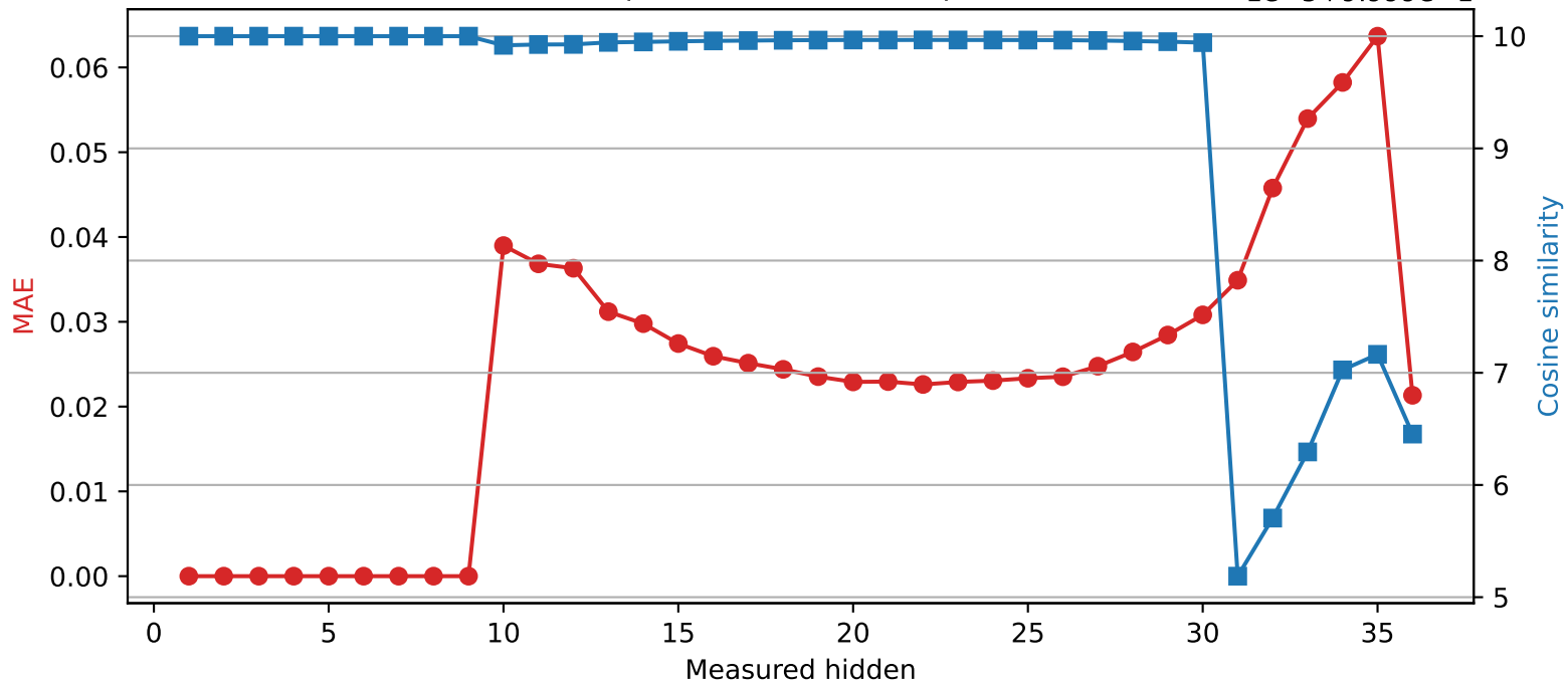
Qwen2.5-3B | Quantized layer 9 | float16 → int8
